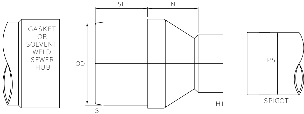
FABRICATED FITTING (F)
